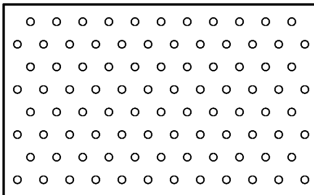
SPECIAL PATTERN P55 (.078 x .270 staggered)
