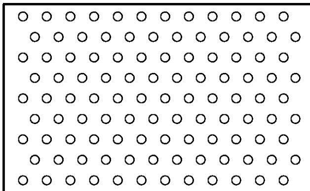
SPECIAL PATTERN P64 (.094 x .250 staggered)
