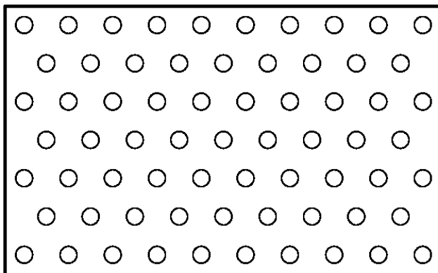
SPECIAL PATTERN P88 (.125 x .328 staggered)
