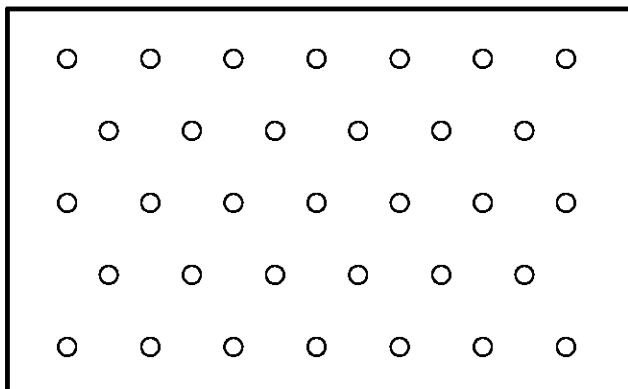
SPECIAL PATTERN P66 (.094 x .433 staggered)
