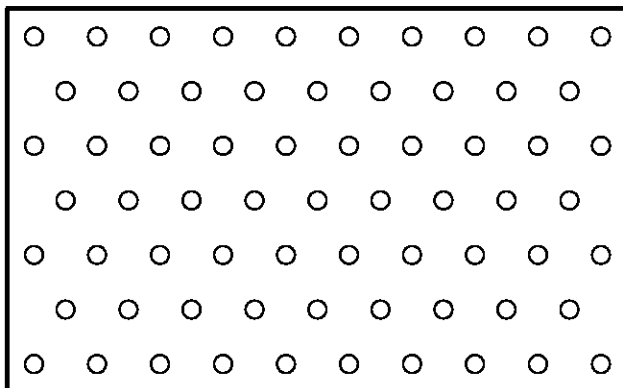
SPECIAL PATTERN P65 (.094 x .328 staggered)
