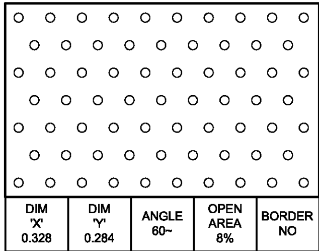
SPECIAL PATTERN P88 (.125 x .328 staggered)
