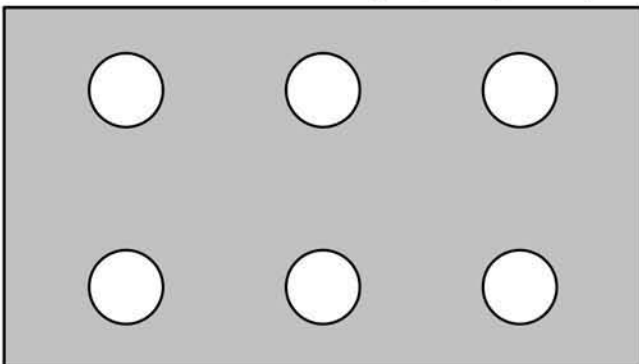
PATTERN P242 (3/8" round, 1" o.c., straights, 11% Open Area)
