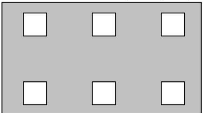
PATTERN P24S1 (3/8" square, 1-1/8" o.c., straights, 11% Open Area)
