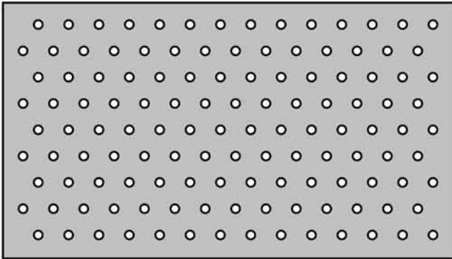
PATTERN P124 (3/16" round, 3/8" o.c., staggereds, 23% Open Area)
