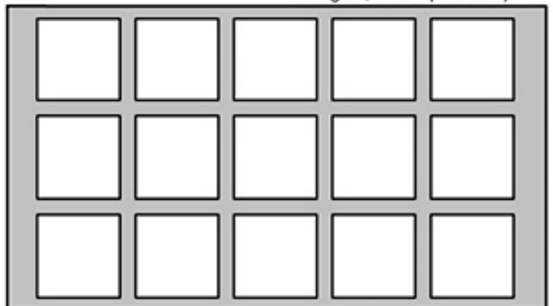
PATTERN P32S2 (1/2" square, 19/32" o.c., straights, 70% Open Area)
