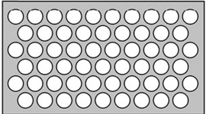
PATTERN P163 (1/4" round, 5/16" o.c., staggereds, 58% Open Area)
