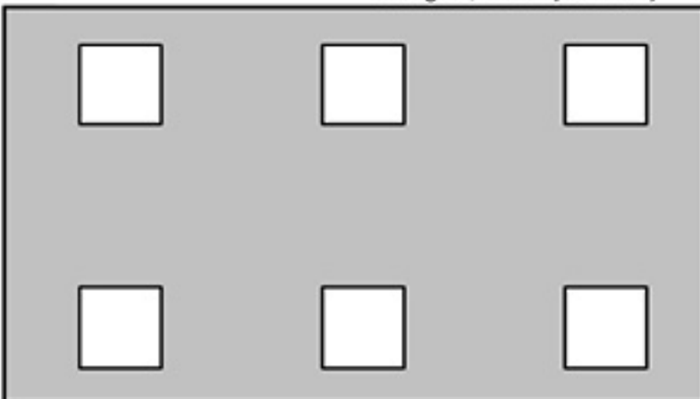
PATTERN P24S1 (3/8" square, 1-1/8" o.c., straights, 11% Open Area)
