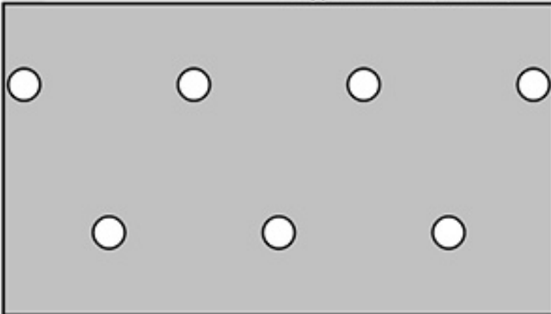
PATTERN P126 (3/16" round, 1" o.c., staggereds, 4% Open Area)
