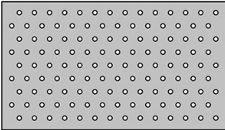
PATTERN P124 (3/16" round, 3/8" o.c., staggereds, 23% Open Area)
