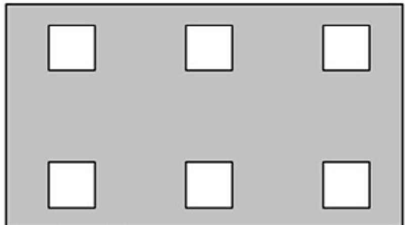
PATTERN P24S1 (3/8" square, 1-1/8" o.c., straights, 11% Open Area)
